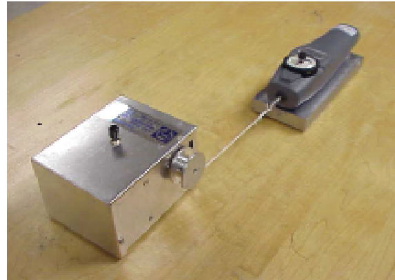
Figure 1. The Horizontal Pull Slipmeter (HPS) 5
