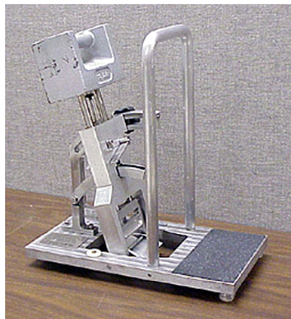
Figure 2. The Brungraber Mk II 6
